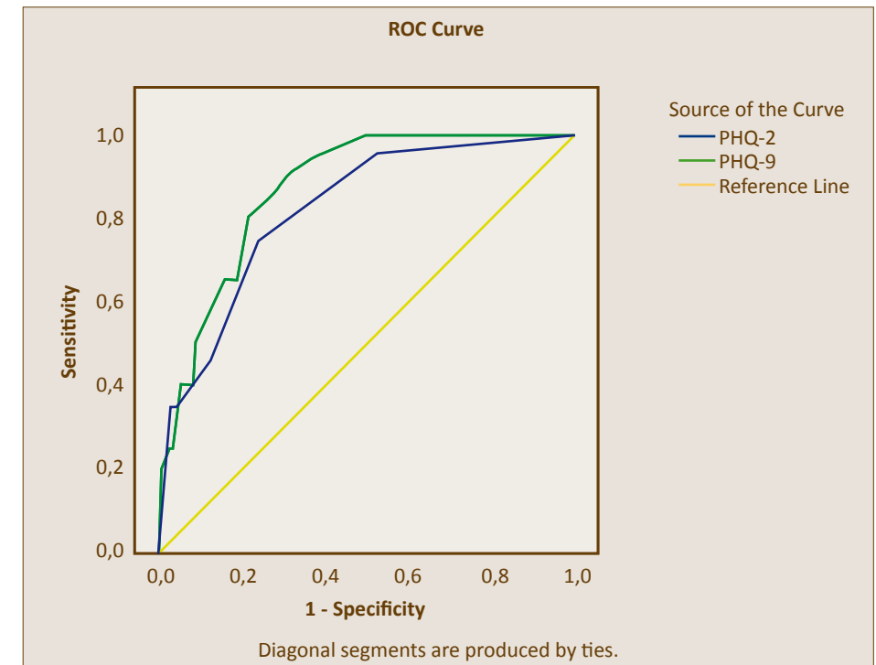
Figure 2. ROC PHQ-9 and PHQ-2 versus CIDI scores
